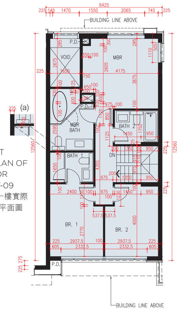
1st FLOOR PLAN 一樓平面圖
